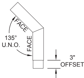
STYLE 2 ELBOW
