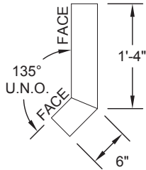
STANDARD ELBOW
