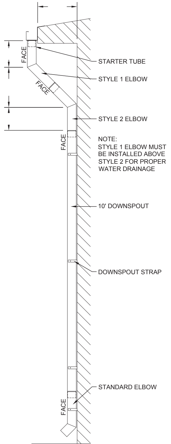
STARTER TUBE
