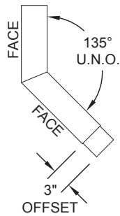
STYLE 1 ELBOW
