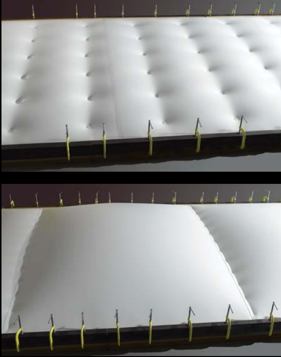
The RhinoBond welded membrane spreads the wind load evenly across the roof (top) as opposed to the traditional in-seam fastening method (bottom).
