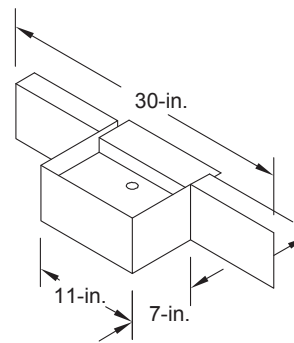
SUMP 2 PIECE ASSEMBLY
