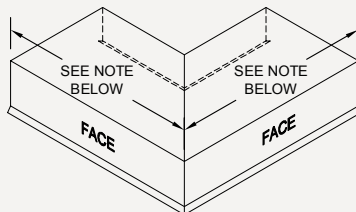
OUTSIDE MITER
